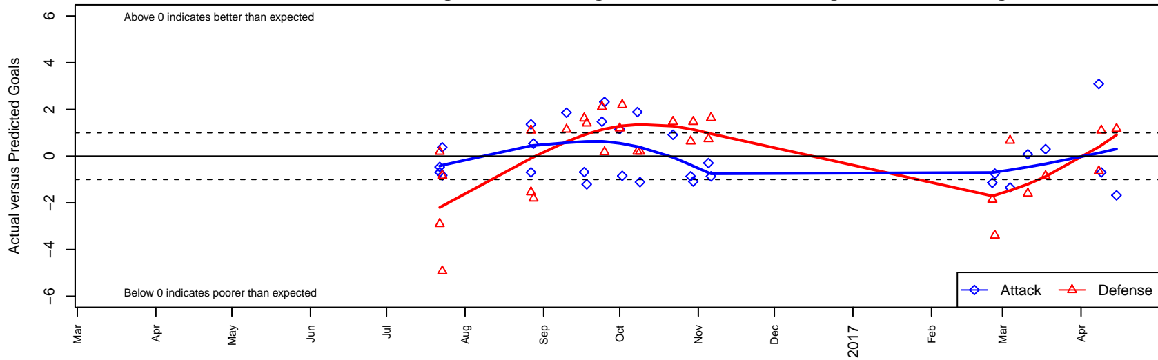
THUSC Nitrogen Black G05 Dots are actual minus expected GF (blue circles) and GA (red triangles). Blue line is smoothed change in attack strength. Red is smoothed change in defense strength.
